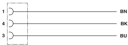
Contact assignment of M8 plugs/sockets
